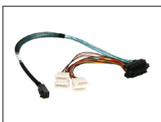
K-HD43X82-50 HD miniSAS SFF-8643 to 4x SFF-8482 50 cm Cable
